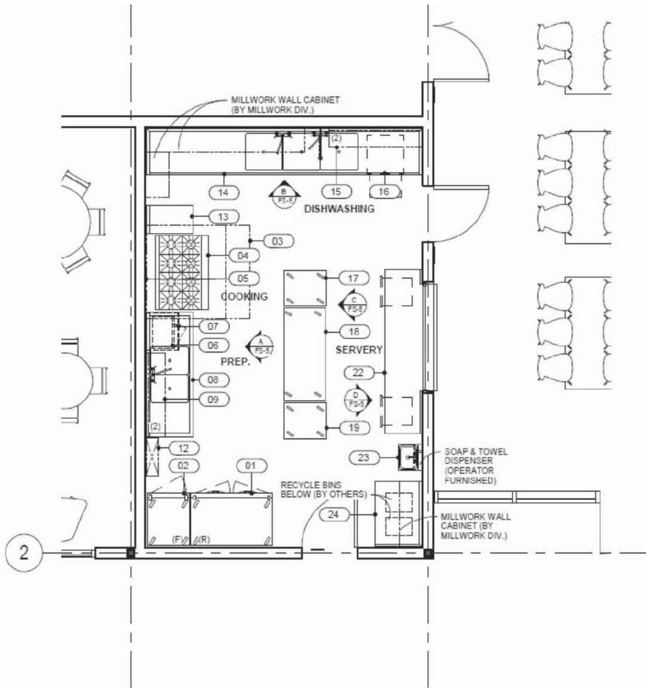
1 EQUIPMENT PLAN 1/4" = 1'-0"
