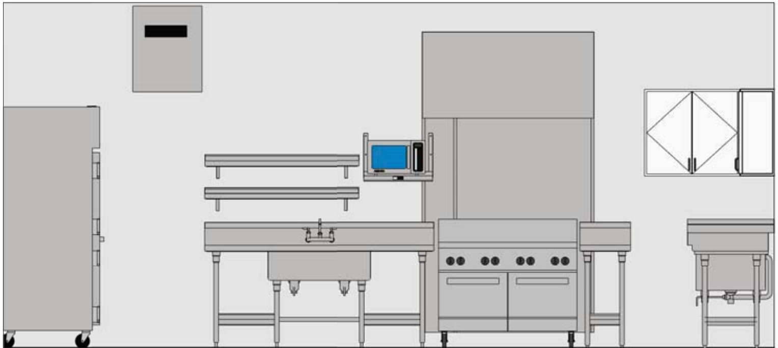
WEST ELEVATION
