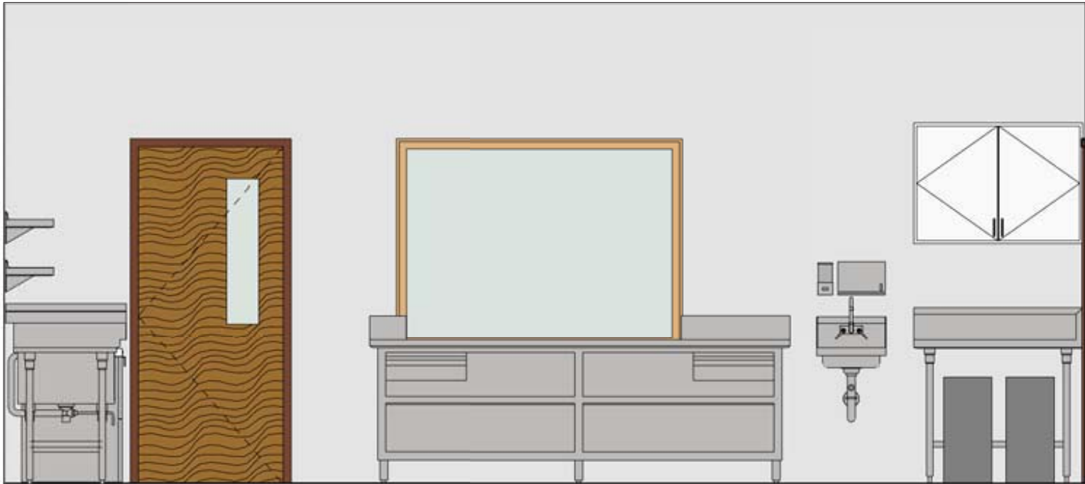
EAST ELEVATION
